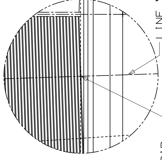
DETAIL F SCALE 20/1
