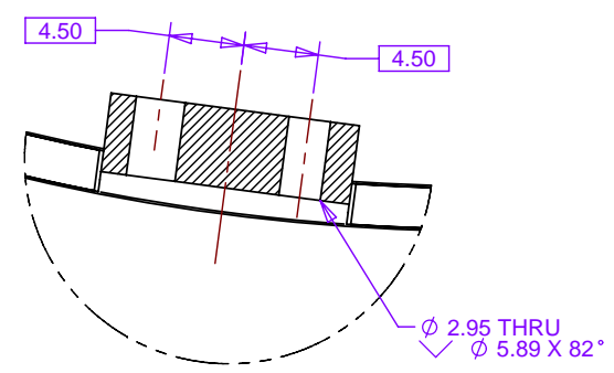
DETAIL E SCALE 4 : 1 VIEW TYP 3X
