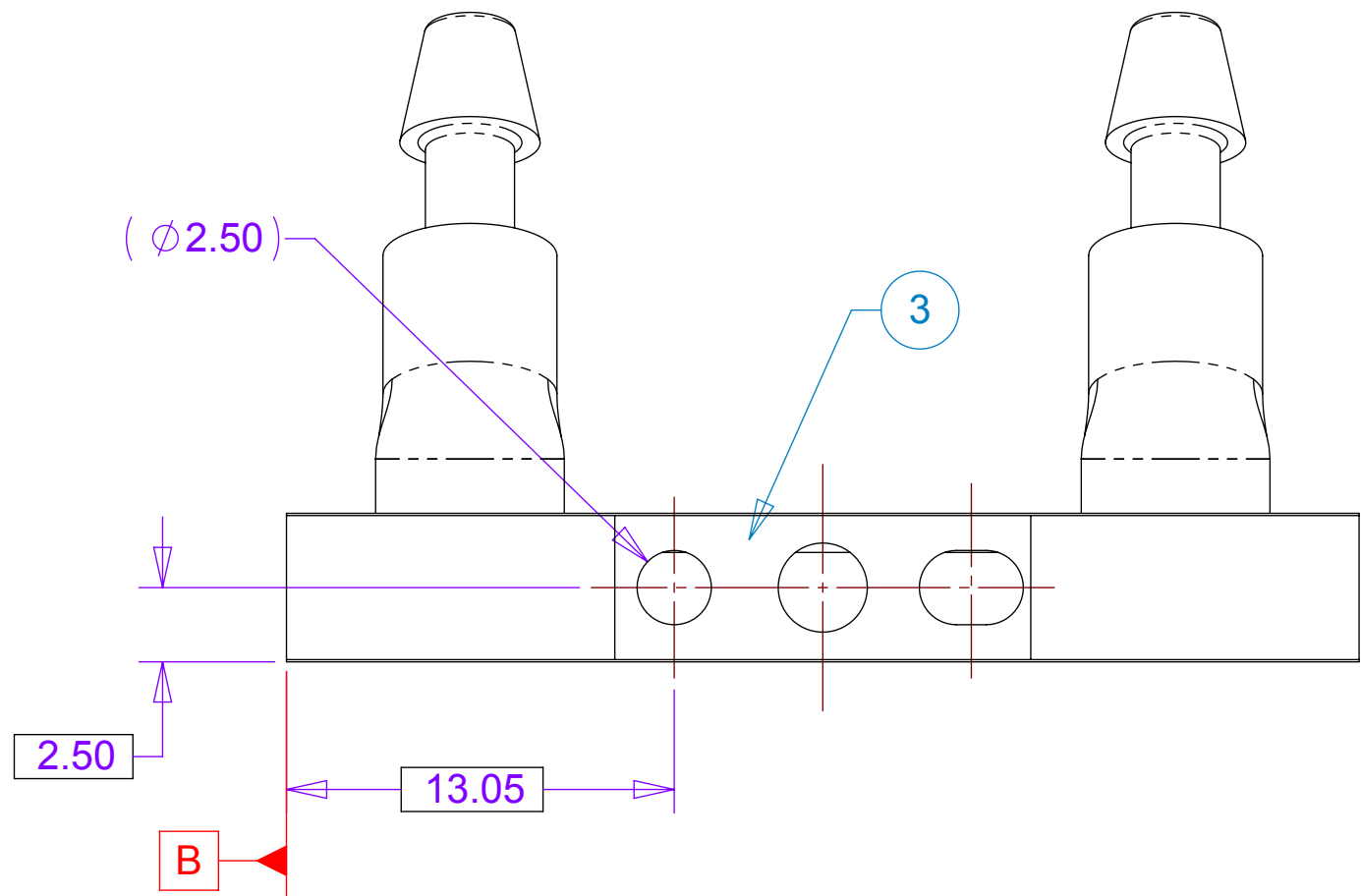
SECTION B-B
