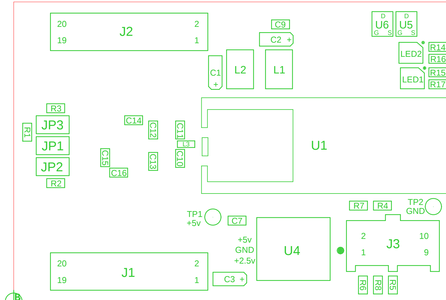
126Y-267911 REV0 ASSY. (TOP)
