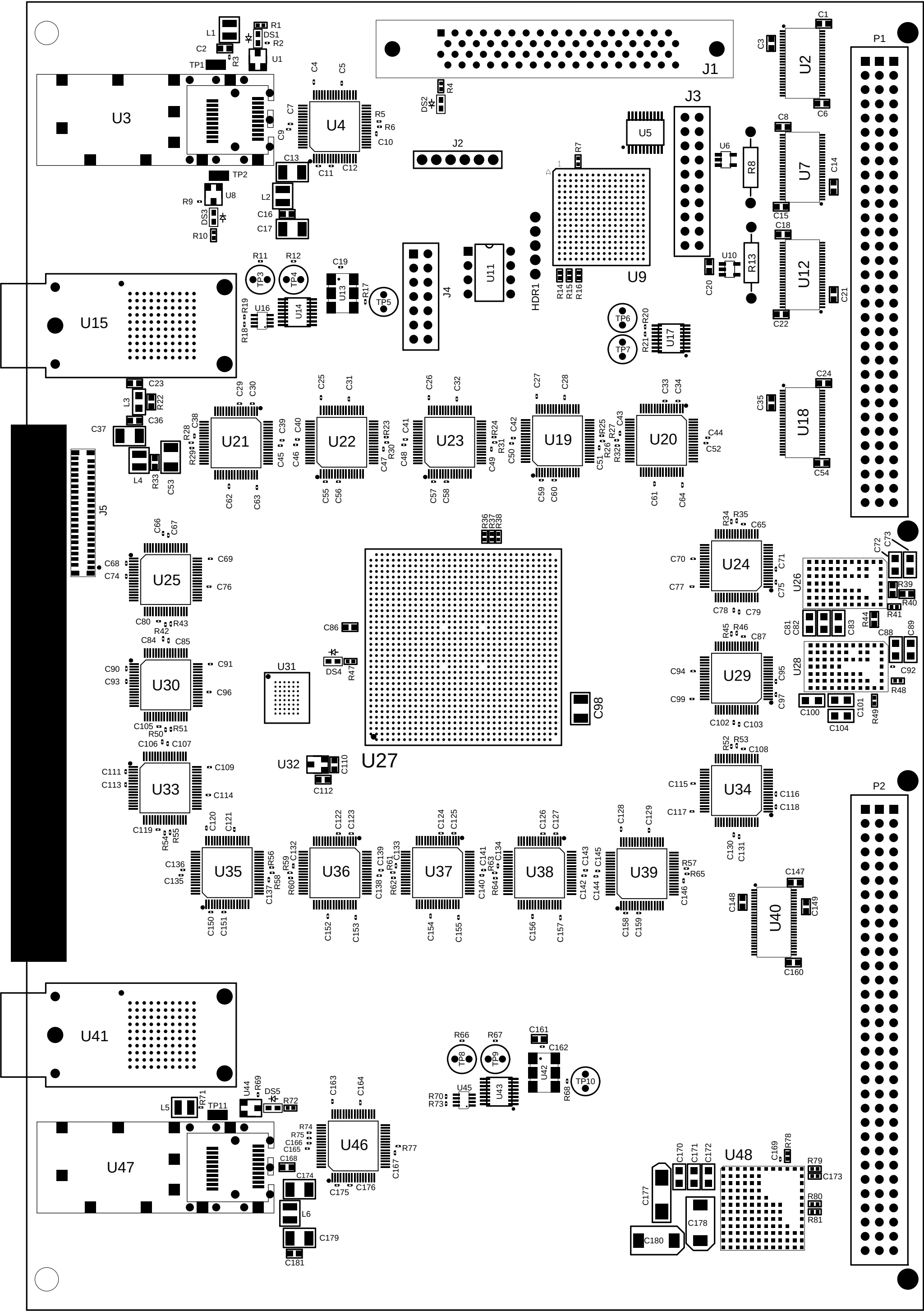
126Y-267961A ASSEMBLY - PRIMARY SIDE
