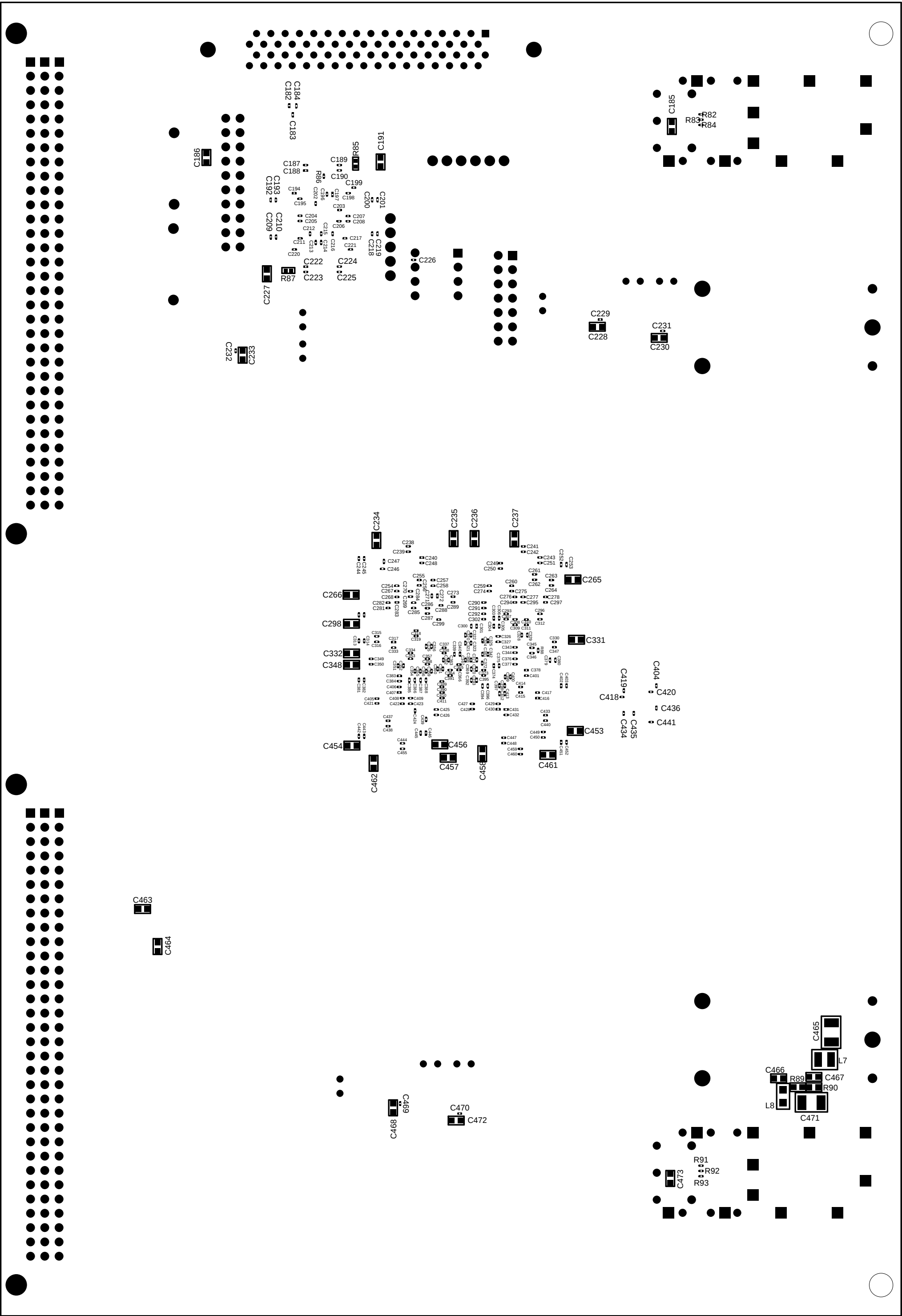
126Y-267961A ASSEMBLY - SECONDARY SIDE
