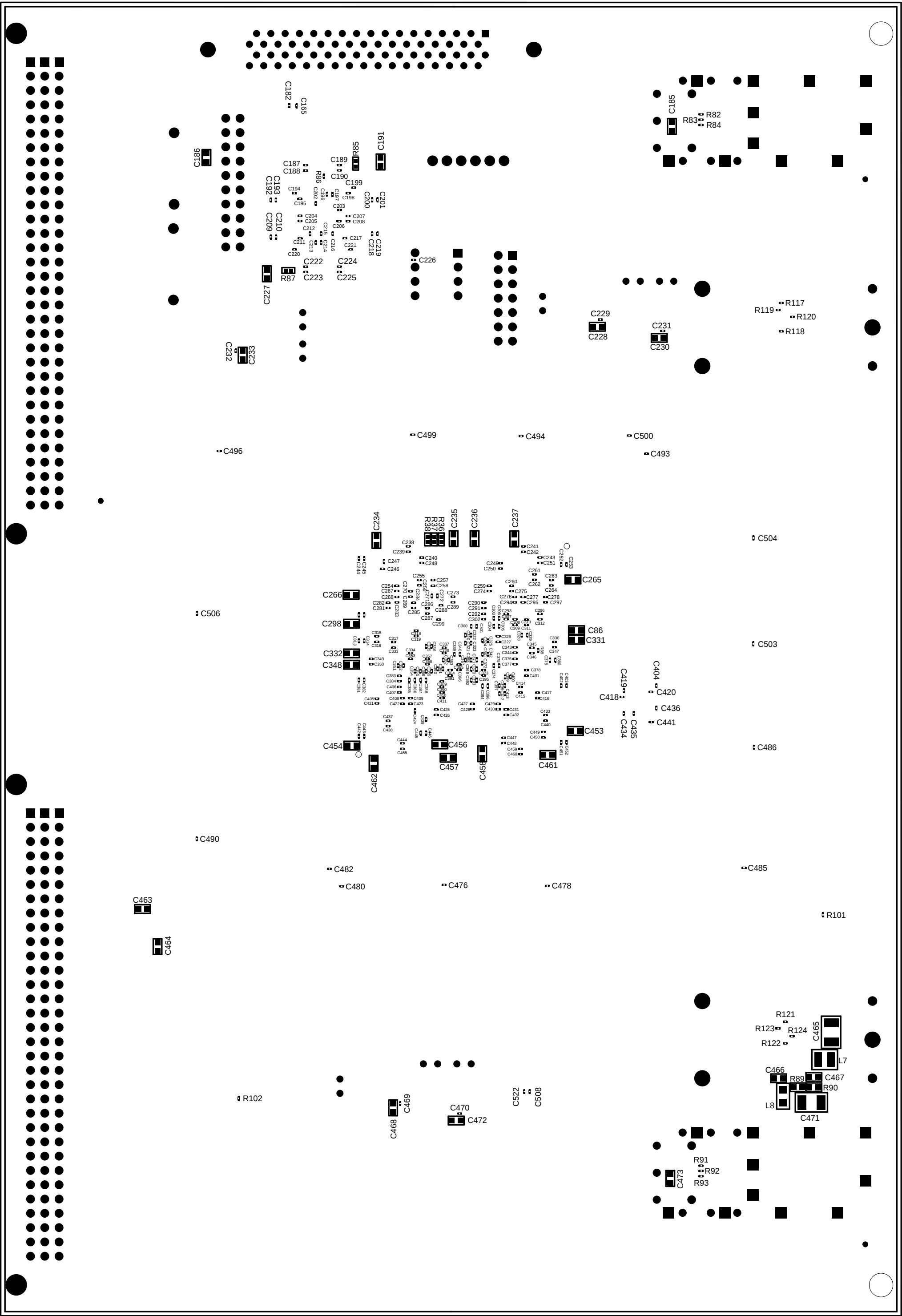
126Y-267961B ASSEMBLY - SECONDARY SIDE
