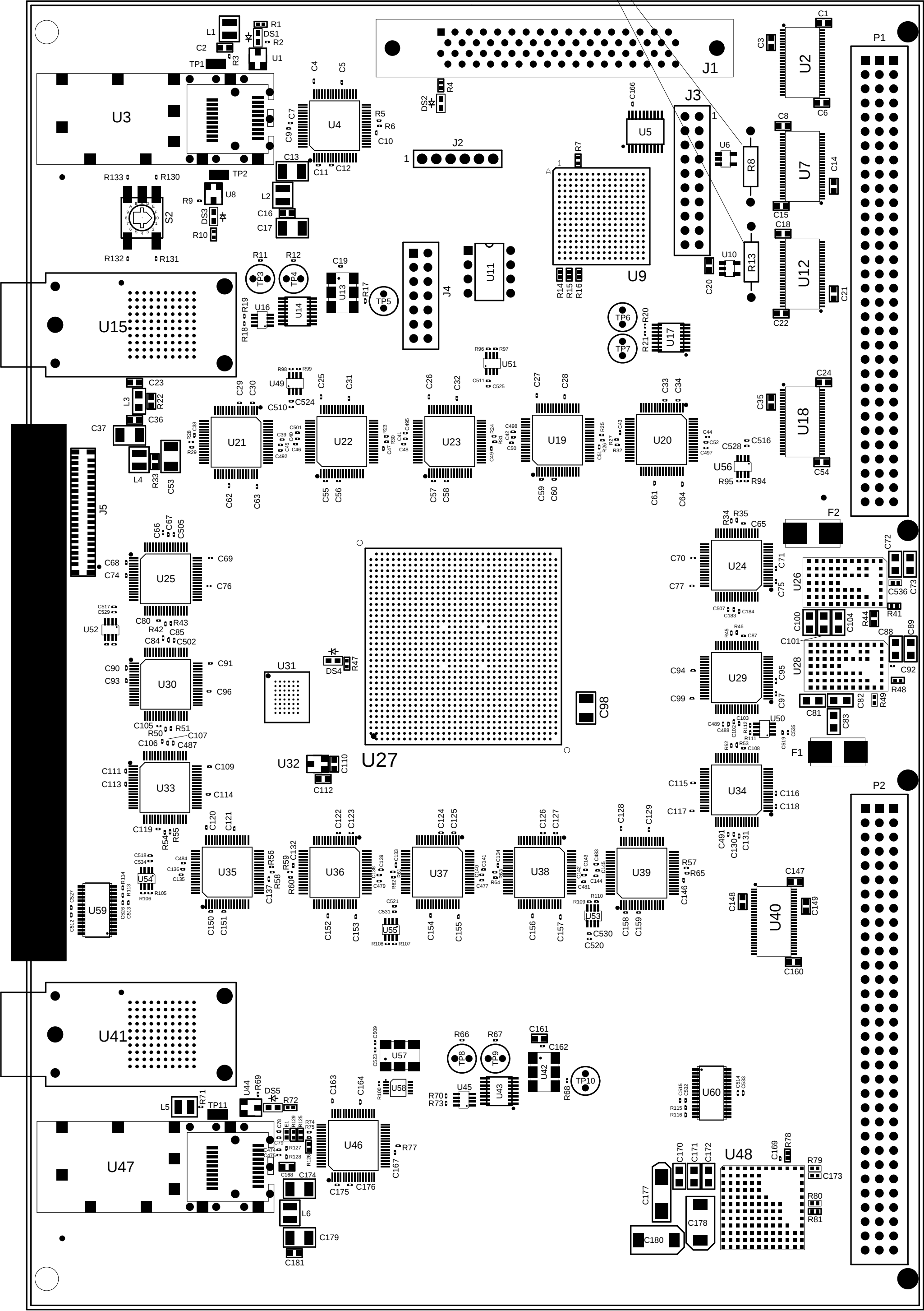
126Y-267961B ASSEMBLY - PRIMARY SIDE
