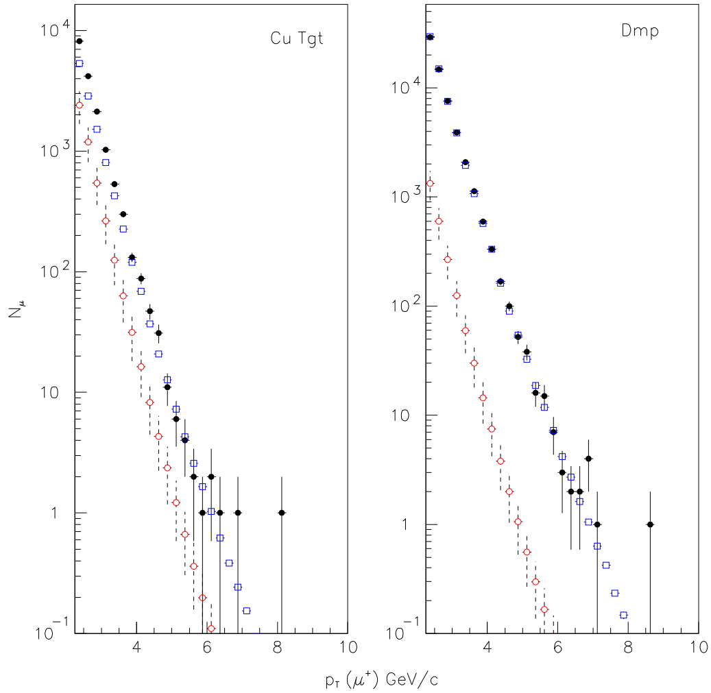
Figure 5.2: Total open charm Monte Carlo \mu^+ contribution (blue open squares), total light MC \mu^+ spectra from Figure 5.1 (red open circles) and the the data (black filled circles) from the copper target (left) and the dump (right). Data is the \mu^+ spectra from the copper target, and the Monte Carlo spectra are from fitting the 3 variable function with n a free parameter. Data errors are statistical only. MC spectra have all systematic errors except normalization added in quadrature to the statistical error.
