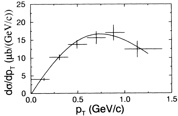
Figure 1.5: Differential cross section per nucleon, d\sigma(D^0) / dp_T + d\sigma(\bar{D}^0) / dp_T versus p_T . Uncertainties shown are statistical only and do not include an additional systematic uncertainty of 12.8 percent. Figure is from Fermilab Experiment 789[8].
