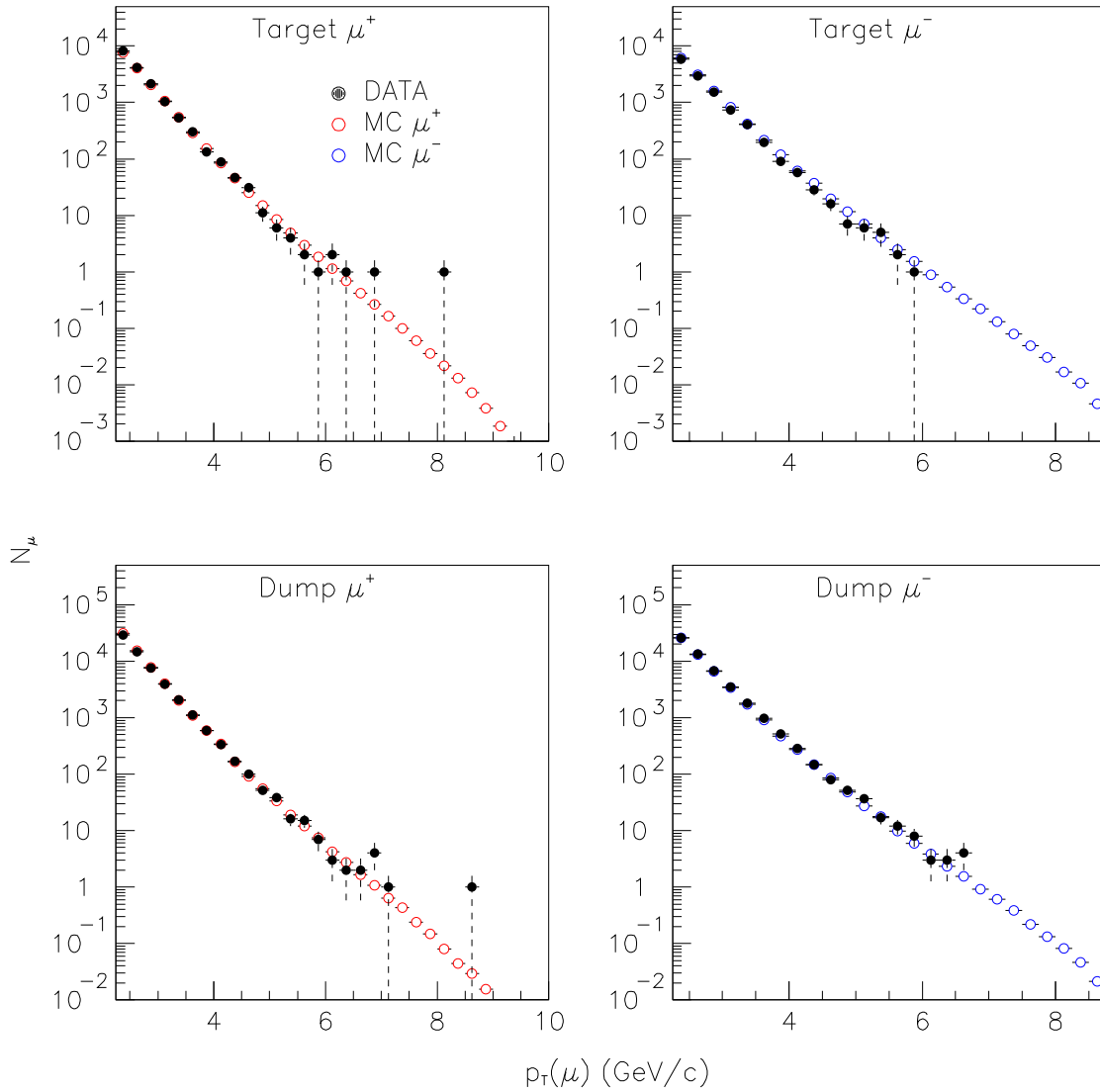
Figure 6.4: The copper target data (black closed circles) and total Monte Carlo spectra at \chi^2_{min} (red open circles) from the fit where the D/\bar{D} cross sections were of the form \frac{A_2}{(p_T^2 + \alpha m_c^2)^n} . The exponent n was a free parameter for this fit. Histograms are \mu^+ (left) and \mu^- (right) for the copper target (top) and copper dump (bottom). Errors for the data are statistical only. Errors for the Monte Carlo include all errors used for calculating \chi^2 (see text). Error bars may be smaller than symbols used.
