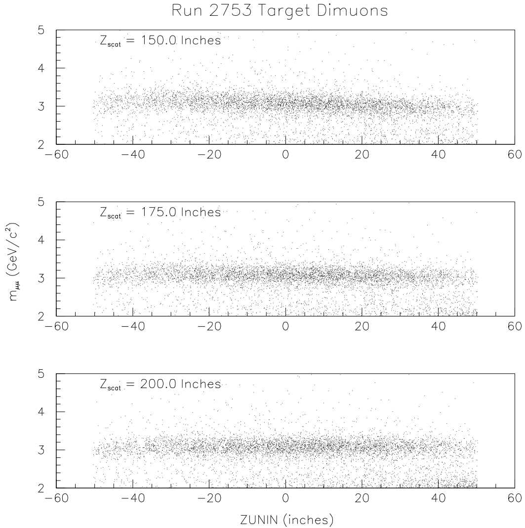
Figure 3.7: Reconstructed dimuon mass, m_{\mu\mu} (GeV c^{-2} ), versus the estimated z vertex (inches) for the target analysis of Run 2753. All plots use the same spectrometer calibrations except the position for the scattering bend plane, Z_{scat} , which was set to 150.0 inches for the top plot, 175.0 inches for the middle and 200.0 inches on bottom. Plots were used to determine the optimal position resulting in the minimum width of the mass spectrum, which occurred when there was no slope.
