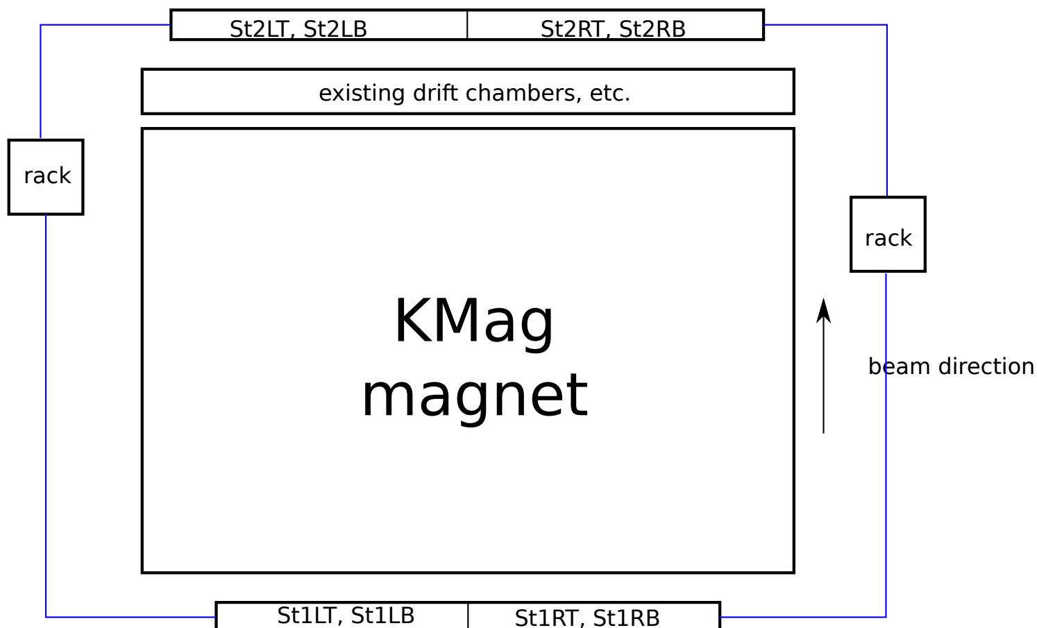
overall plan (viewed from above)
